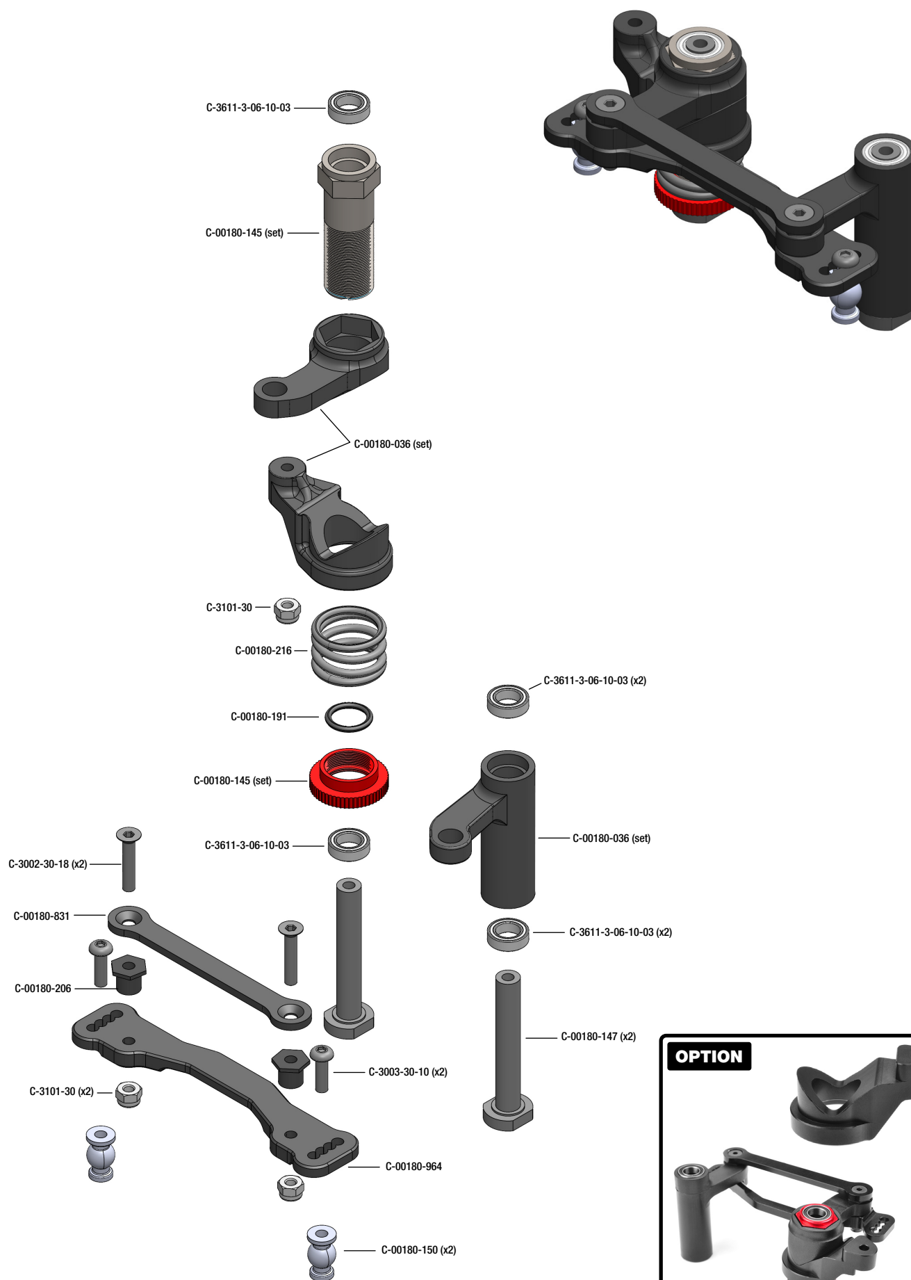
C-00180-266 Servo Saver Steering Arm - 7075 T6 - Hard Anodised - Black - 1 pc
